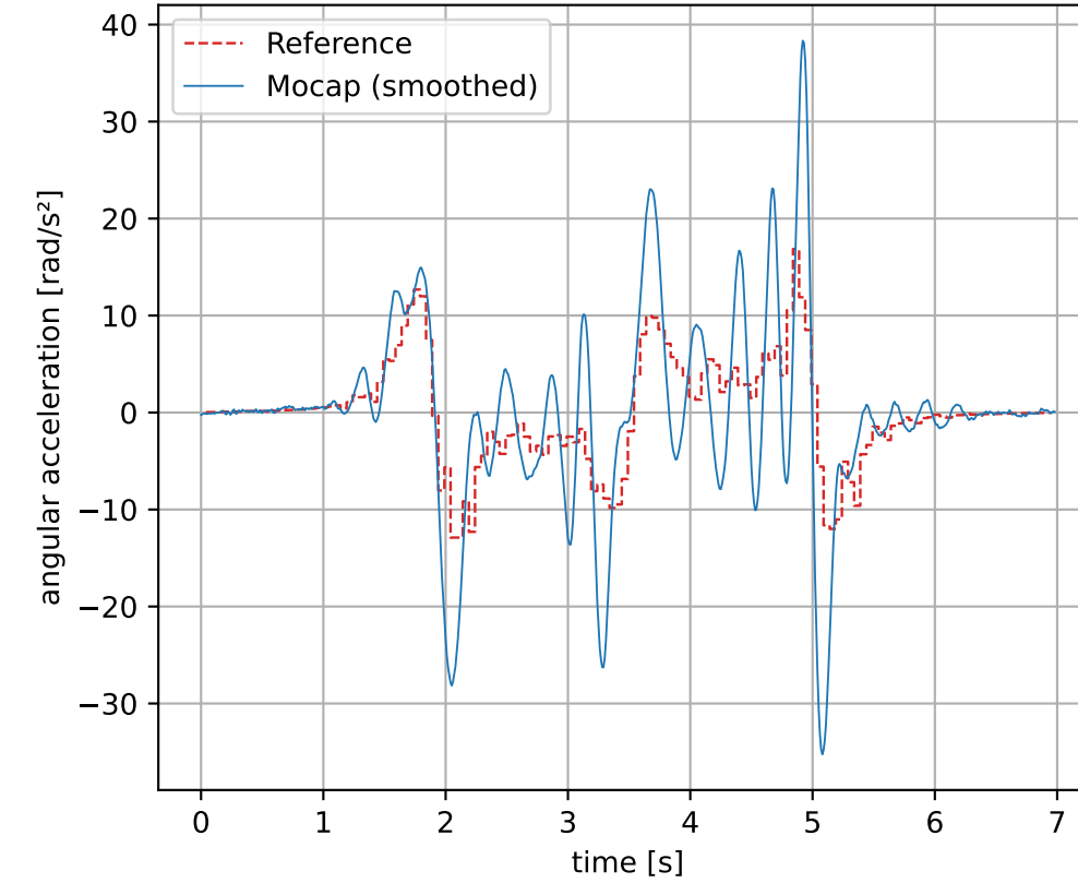
Angular Acceleration
